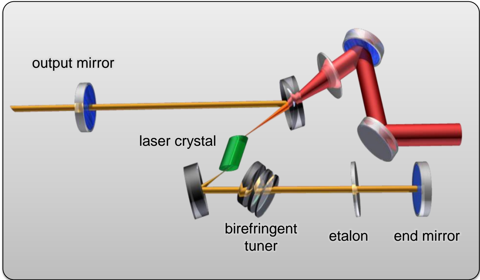
Standard Ti:Sa cavity design
